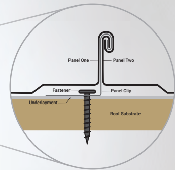
Enlarged Clip Assembly
